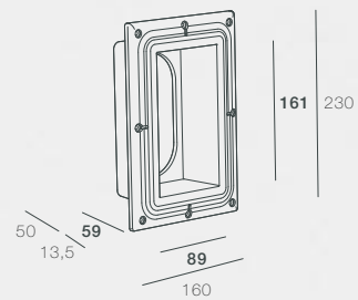
PJ-SMOOTH-02-ST (Frame only)
