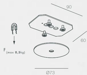
□ PJ-WAY-OUT set L1 WS
