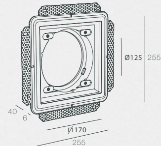
PJ-AERO-S-SQ-ST (Frame only)
