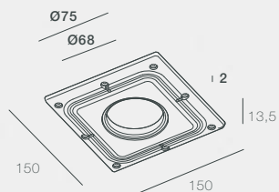
PJ-WAY-OUT-HW (Frame only)
