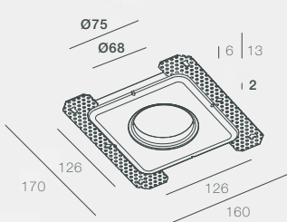
PJ-WAY-OUT-ST (Frame only)
