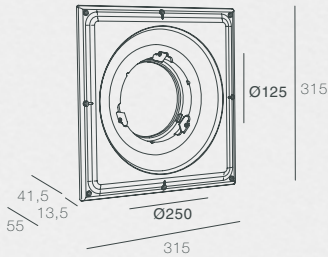
PJ-AERO-M-R-ST (Frame only)
