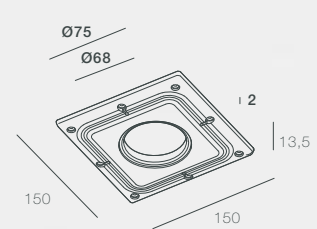
PJ-WAY-OUT-HW (Frame only)
