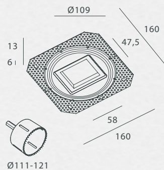
PJ-F-LS-DOTS-ST (Frame only) - Conversion kit for Light Shadow Dots (Compatible with Single frame - Flos ref: 08.0580.00)
