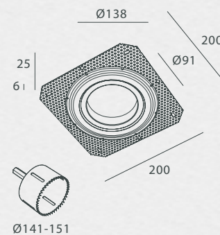
PJ-F-LS-60-A-ST (Frame only) - Conversion kit for Light Shadow 60 Adjustable (Compatible with Flos Ref: 08.0166.00)
