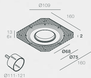
PJ-WAY-OUT-R-ST (Frame only)
