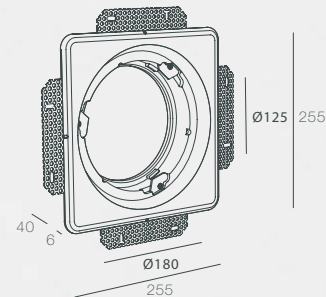
PJ-AERO-S-R-ST (Frame only)
