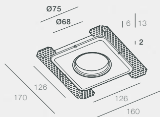
PJ-WAY-OUT-ST (Frame only)
