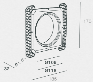
PJ-PHANTOM-Twist-ST (Frame only)
