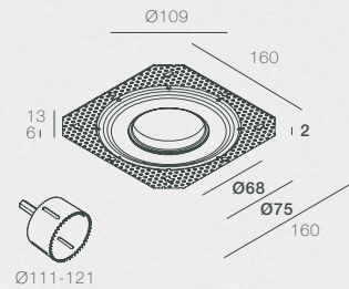
PJ-WAY-OUT-R-ST (Frame only)
