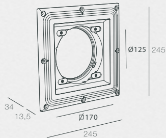
PJ-AERO-S-SQ-ST (Frame only)
