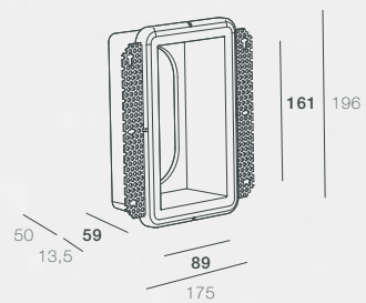
PJ-SMOOTH-02-ST (Frame only)
