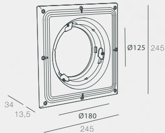
PJ-AERO-S-R-ST (Frame only)
