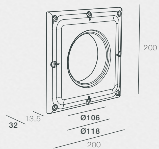
PJ-PHANTOM-Twist-ST (Frame only)
