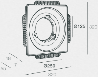
PJ-AERO Collar Ø 125 PJ-AERO-S-R-FELT AIR VENTIL
