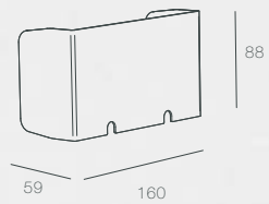
□ PJ-SMOOTH CV-LV WS
